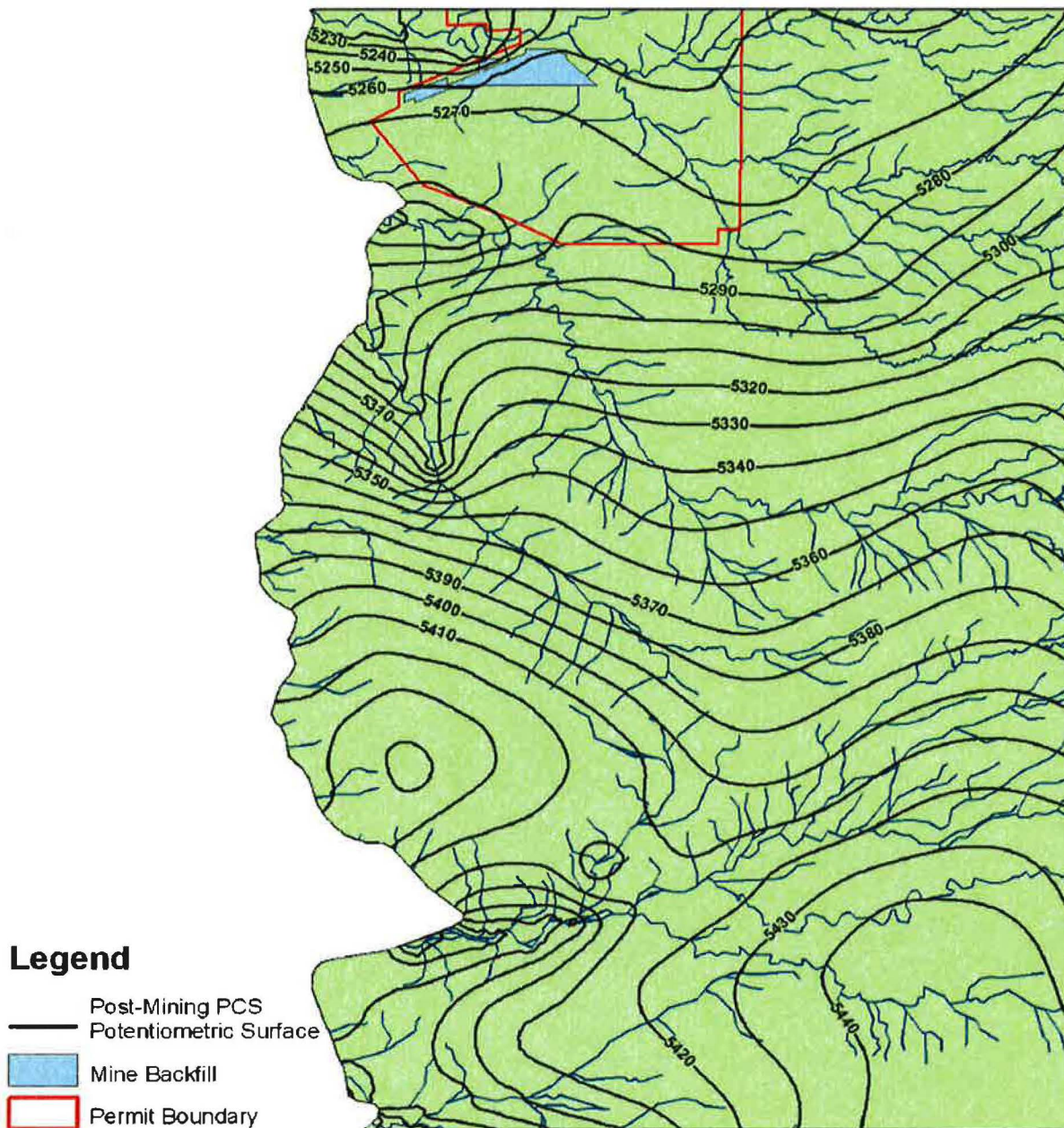
Figure 32: Post-Mining Potentiometric Surface in the PCS Aquifer (NTEC 2013)
